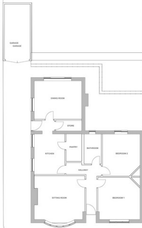
GROUND FLOOR - 1:50 @A1
